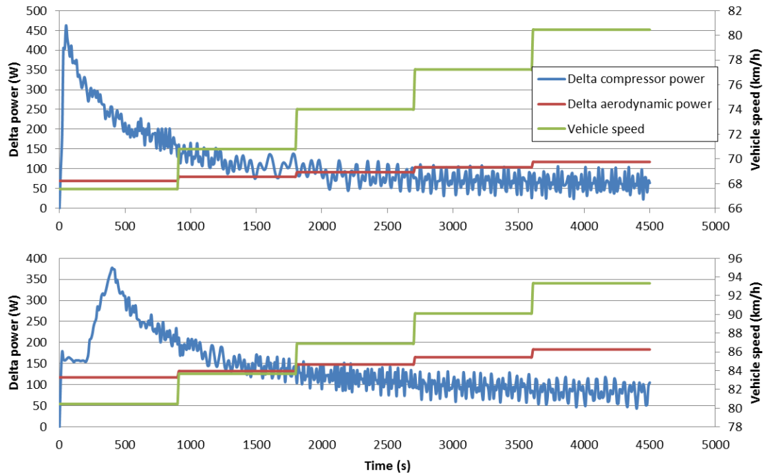
Figure 4-9: The tradeoff between the delta compressor power and the delta aerodynamic power at 26.7°C and 32.2°C. The figure on top shows the result at 26.7°C.
