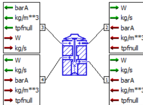
Figure B- 11: AMESim sub-model ACTEVS02 can be used to model the thermostatic expansion valve with an integrated thermal sensing bulb [26].
