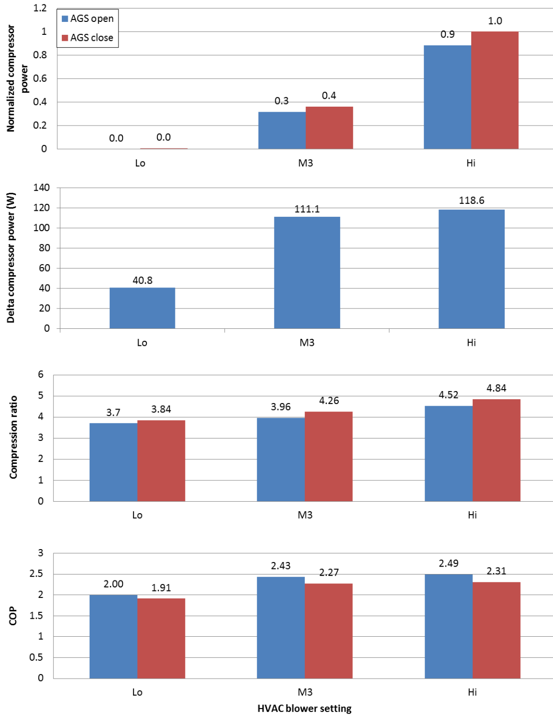
Figure 4-4: Steady-state simulation results at 32.2 °C. The first figure shows the compressor power, the values are normalized according to equation 4-4. The second figure shows the delta compressor power by comparing AGS closed with AGS open condition. The third figure shows the compression ratio and followed with the coefficient of performance (COP).
