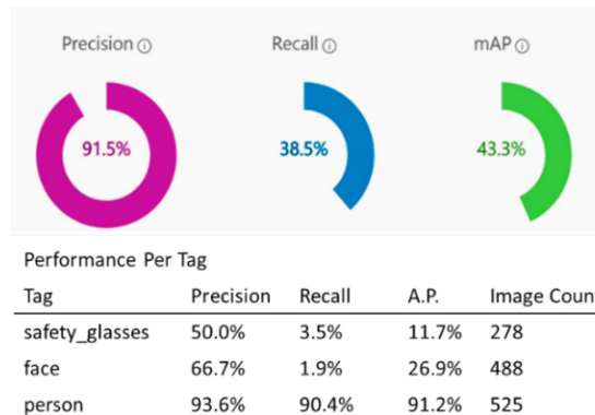
Figura 2.8: Prestazioni Learning Factory: custom dataset.
