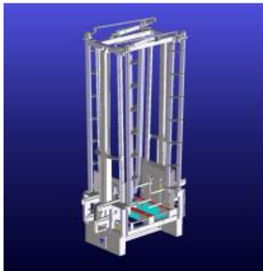
Fig 13. Unstacker with 4 forks
