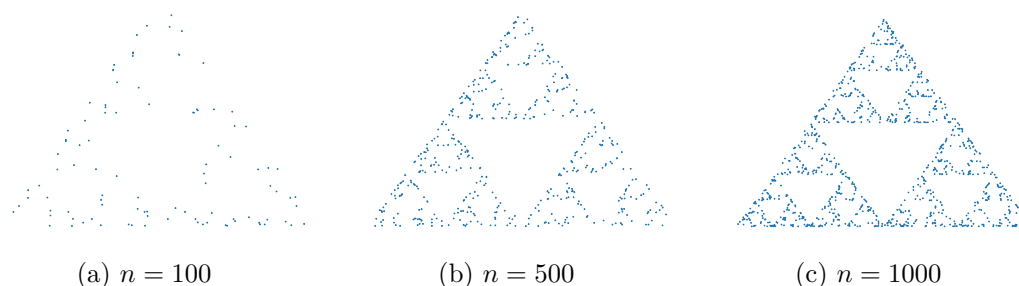
Figure 3.9: Python reproduction of chaos game with varying iterations.
