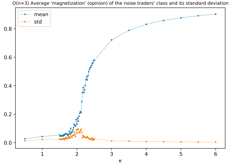
Figure 5.1: Time-average and standard deviation of the magnetization (norm of the mean spin vector of that trading day) of the noise traders class, characterizing the constant kappa simulations for various \kappa values. The model simulated is the O(n = 3) , using the geometric symmetries approach.
