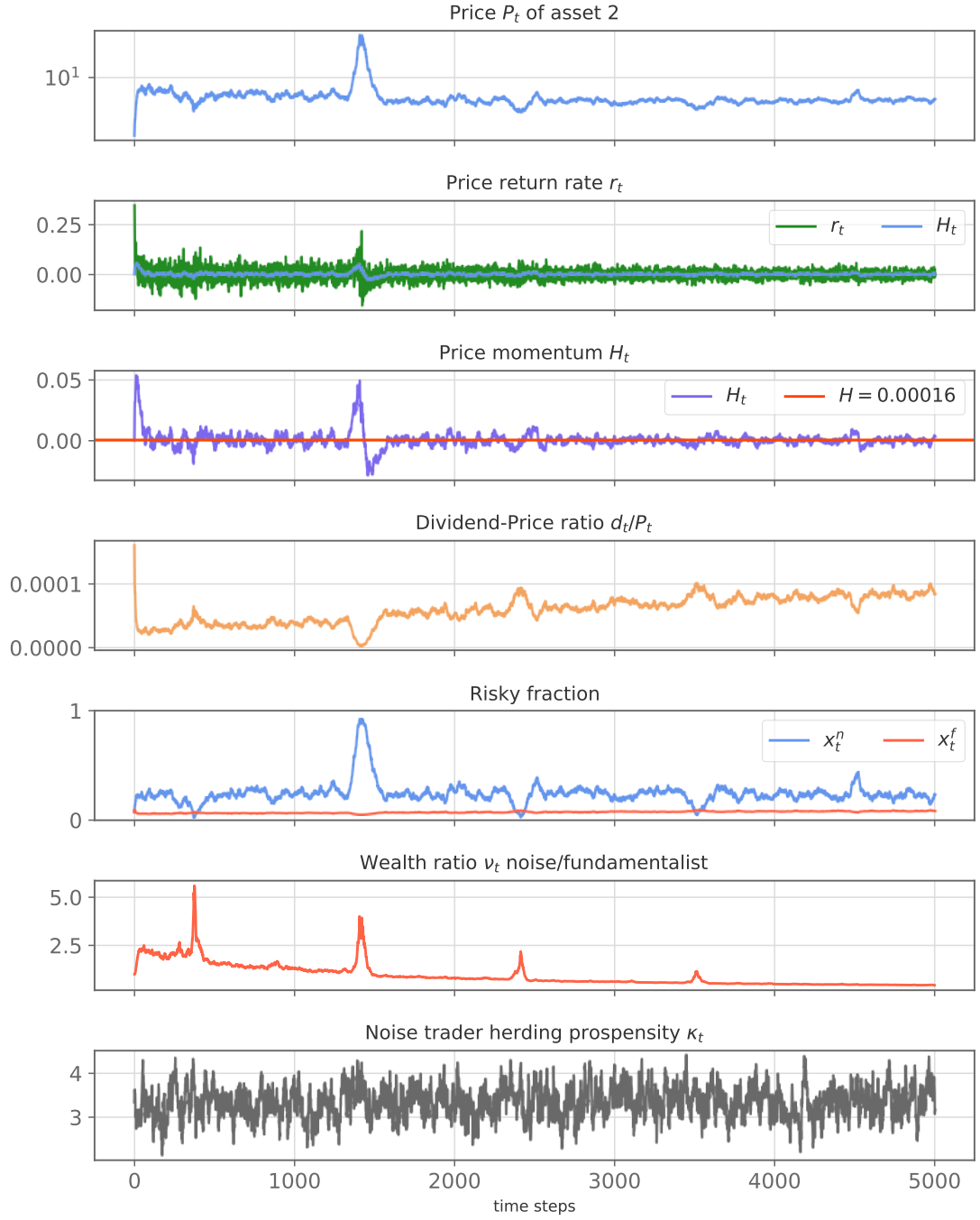
Figure 4.16: Ornstein-Uhlenbeck kappa simulation for the n -state BEG model. The figure shows the detailed time series characterizing the risky asset 2.
