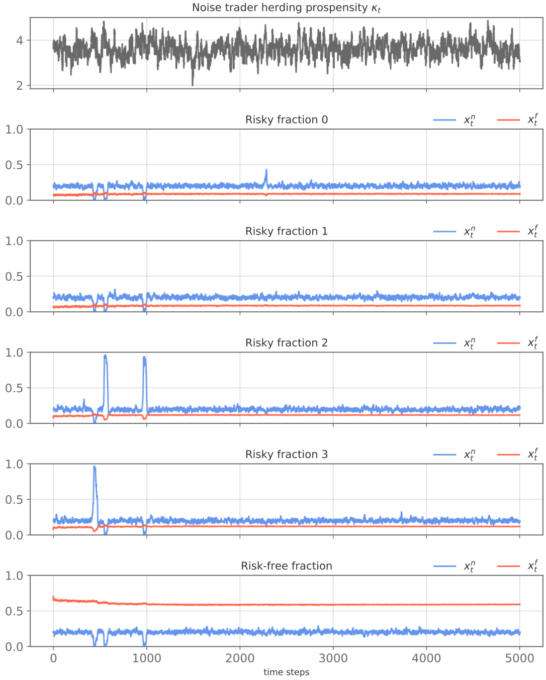
Figure 4.2: Ornstein-Uhlenbeck kappa simulation. The figure shows the time series of the Ornstein-Uhlenbeck kappa process and the time series of both the four risky fractions and the risk-free fraction of the noise traders class at the aggregate level.
