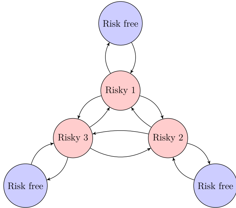
Figure 3.2: Markov chain for the “ n ( n = 3 ) coupled Ising” model
