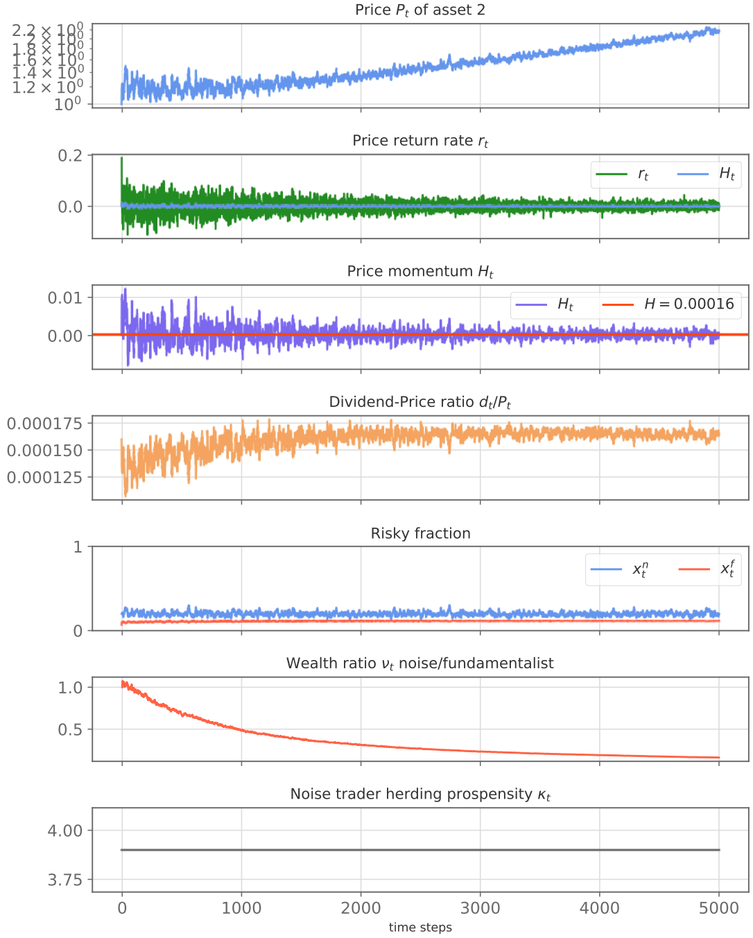
Figure 4.7: Constant kappa simulation. The figure shows the detailed time series characterizing the risky asset 2. No bubble is present.
