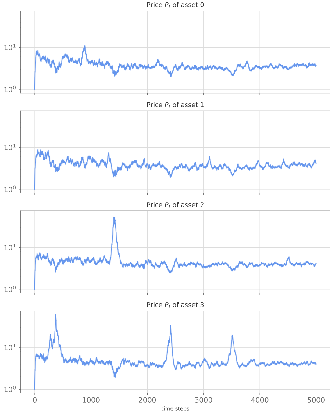
Figure 4.14: Ornstein-Uhlenbeck kappa simulation for the n -state BEG model. The figure shows the time series of the four prices. Several bubbles are clearly identifiable
