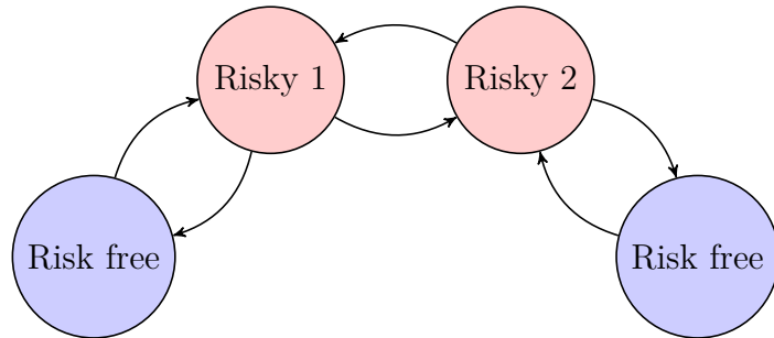
Figure 3.1: Markov chain for the “two coupled Ising” model
