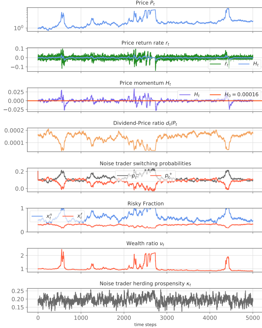
Figure 2.8: Original model Ornstein-Uhlenbeck kappa simulation with linearized rates. The figure shows the time series of the standard implementation of the original model.
