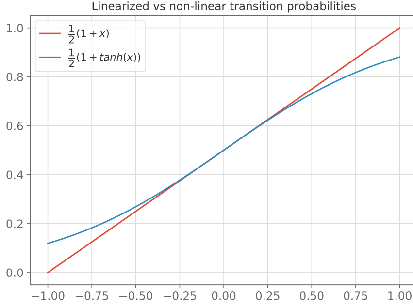
Figure 2.10: Linearized and non-linear forms of the transition probabilities for a range of values x \in [-1, 1] . The two functions clearly differs for relatively large values of the argument, near -1 and 1 .
