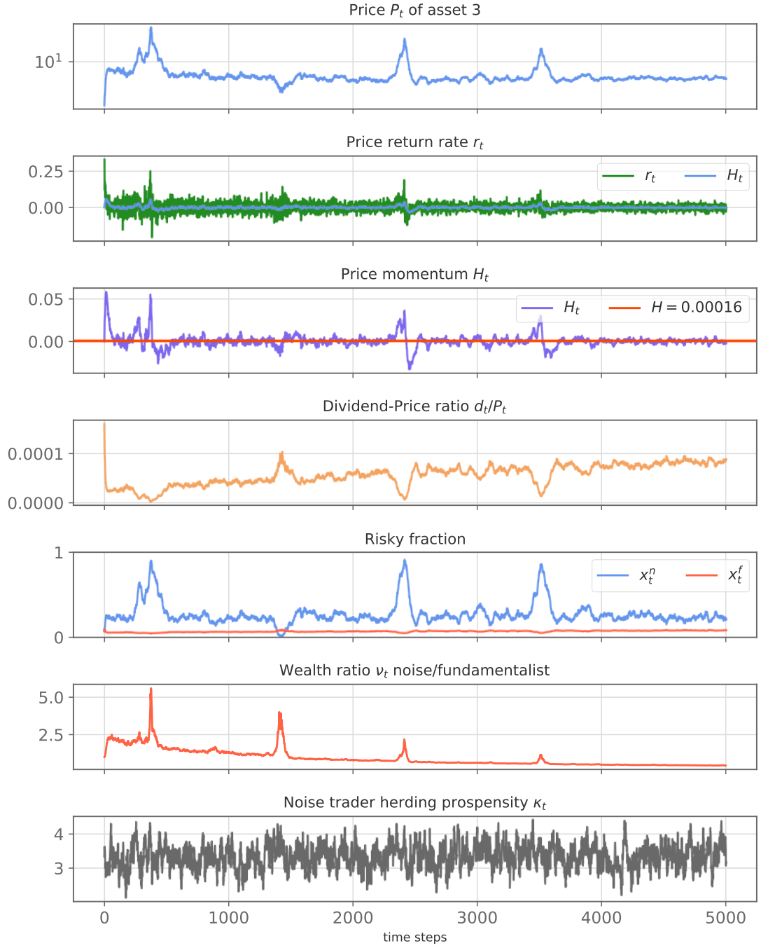
Figure 4.17: Ornstein-Uhlenbeck kappa simulation for the n -state BEG model. The figure shows the detailed time series characterizing the risky asset 3.
