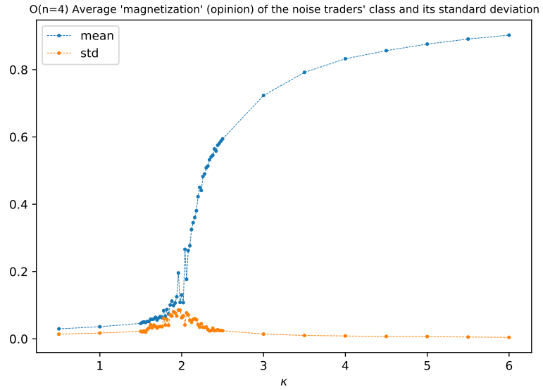
Figure 5.2: O(n = 4) geometric symmetries approach. We refer to figure 5.1 for a detailed description.
