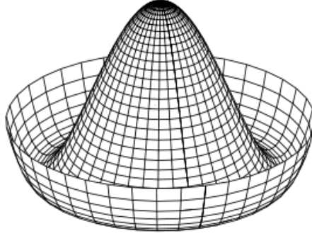
Figure 5.24: Mexican hat potential of the supercritical O(n = 3) model.
