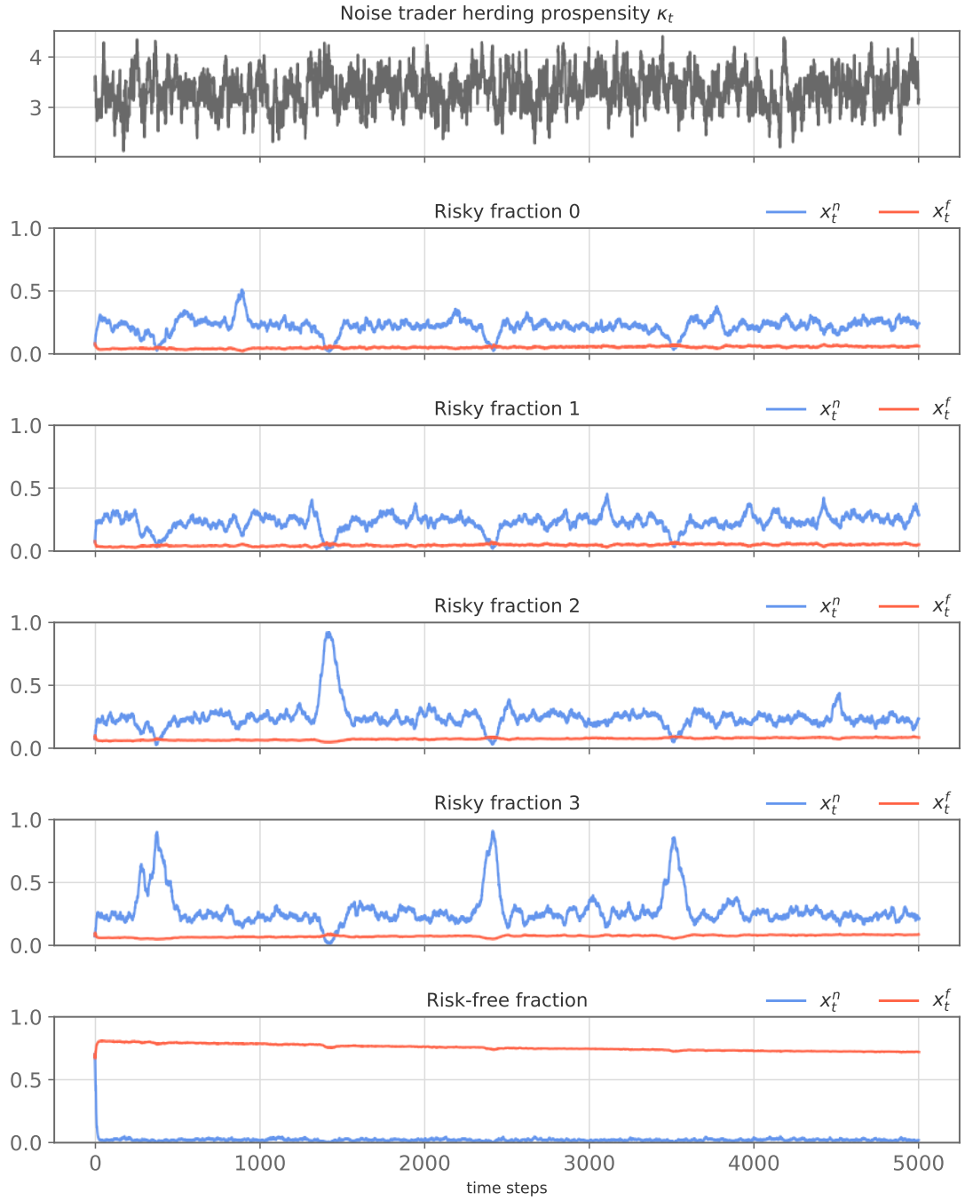
Figure 4.15: Ornstein-Uhlenbeck kappa simulation for the n -state BEG model. The figure shows the time series of the Ornstein-Uhlenbeck kappa process and the time series of both the four risky fractions and the risk-free fraction of the noise traders class at the aggregate level.
