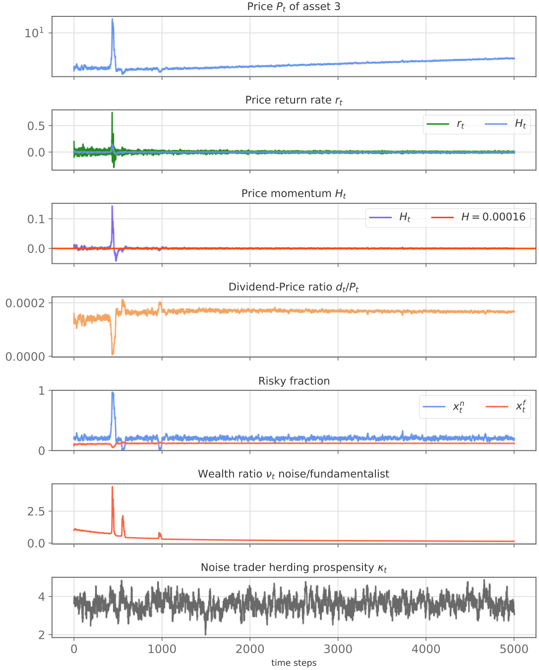
Figure 4.4: Ornstein-Uhlenbeck kappa simulation. The figure shows the detailed time series characterizing the risky asset 3. One bubble is recognizable at the beginning of the simulation.
