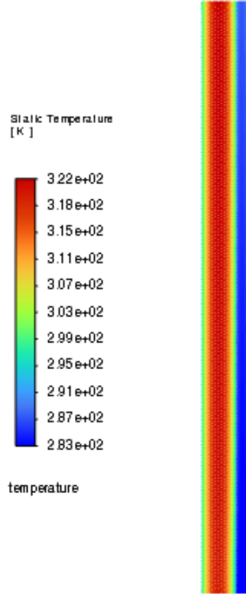
Figure 9: Predicted temperature contour, full domain, Autumn Equinox benchmark case ( d = 0.15 m).
