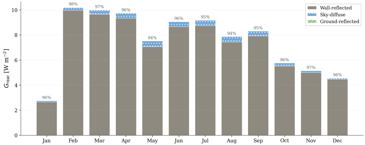
Figure 4: Decomposition of the monthly mean rear-side irradiance of the top module into wall-reflected, sky-diffuse and ground-reflected contributions.
