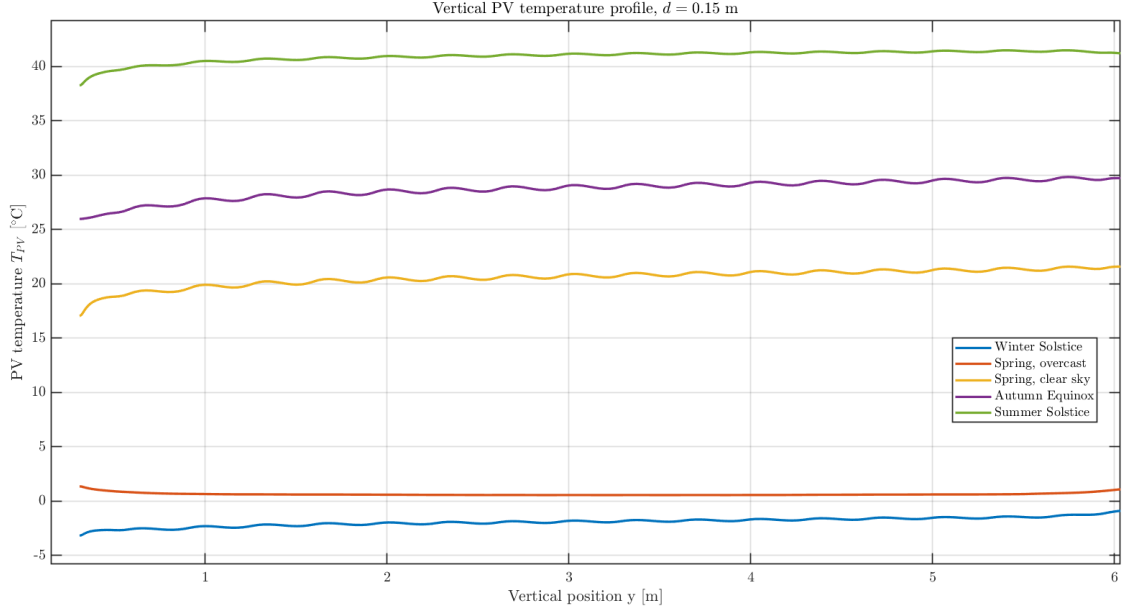
Figure 11: Vertical PV temperature profile along the module column for the five seasonal cases at the baseline gap width ( d = 0.15 m).
