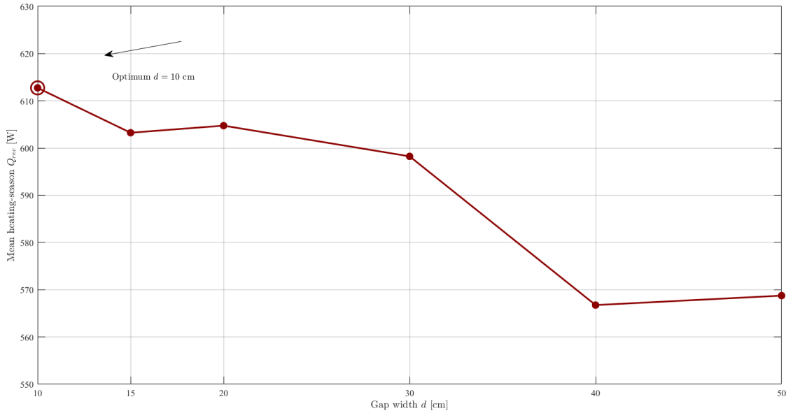
Figure 15: Heating-season mean thermal recovery Q_{rec} as a function of gap width, with the d = 10 cm result highlighted.
