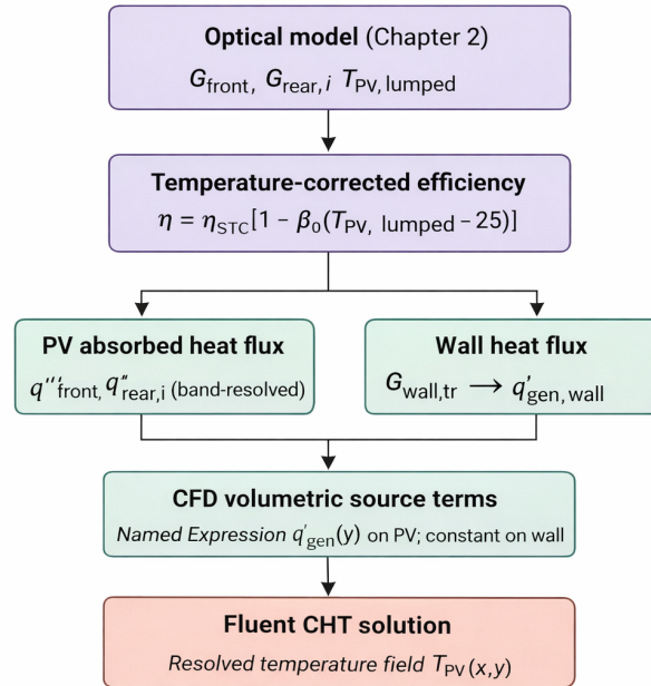
Figure 7: Schematic of the coupling between the optical model (Chapter 2) and the CFD domain: band-resolved irradiance and lumped temperature feed the temperature-corrected efficiency, which determines the PV and wall heat fluxes and hence the volumetric source terms imposed in Fluent. The coupling is one-way: the CFD-resolved temperature field is not fed back into the efficiency correction.
