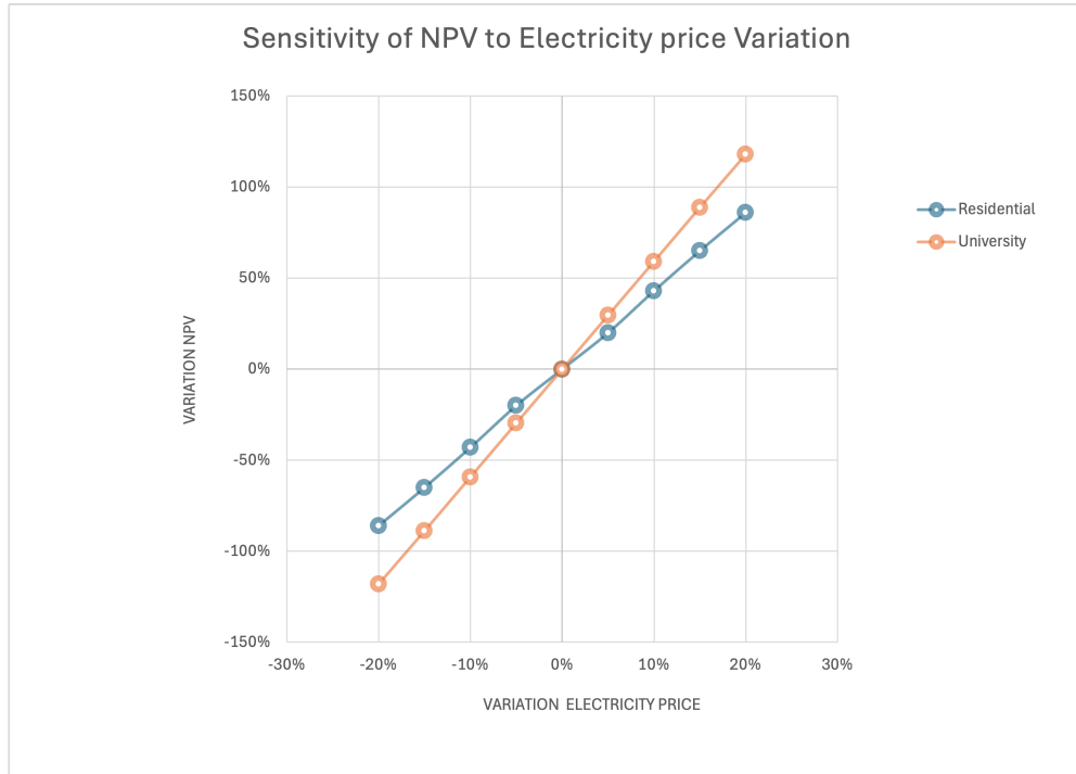
Figure 21: Sensitivity of the NPV to electricity price variations for the university and residential case studies.
