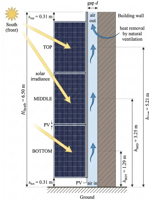
Figure 1: Cross-section of the vertical BIPV façade. Three bifacial modules (TOP, MIDDLE, BOTTOM) are stacked in a contiguous column on the south-facing façade, separated from the building wall by a ventilated air gap of width d . The centre heights of the modules and the overall façade height are indicated.
