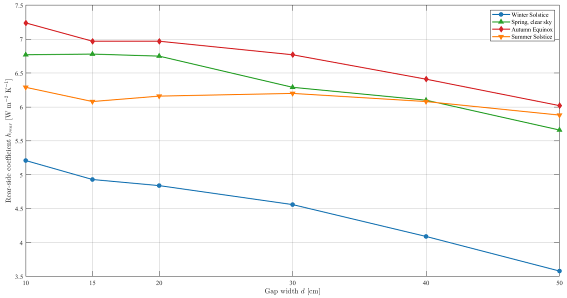
Figure 13: Rear-side convective heat transfer coefficient h_{rear} as a function of gap width, one curve per season (Spring overcast omitted, not significant).
