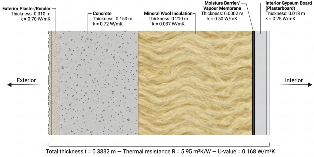
Figure 2: Stratigraphy of the multilayer building wall, from the exterior plaster layer to the interior gypsum board. The equivalent homogeneous wall used in the CFD model preserves the same overall thermal resistance.
