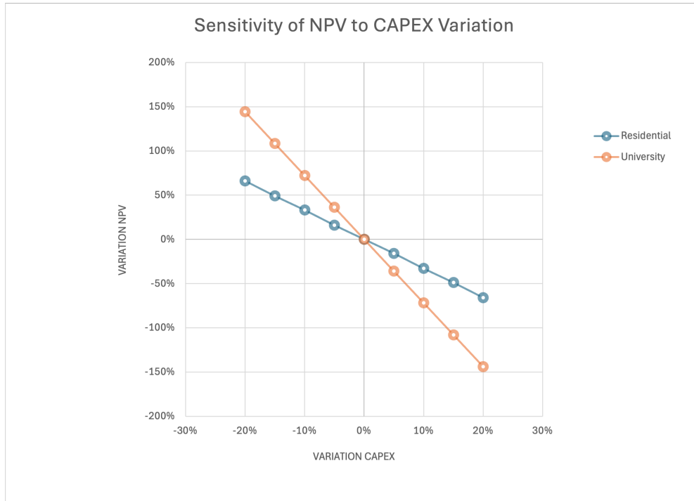
Figure 20: Sensitivity of the NPV to CAPEX variations for the university and residential case studies.
