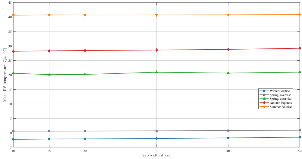
Figure 14: Mean PV temperature as a function of gap width, one curve per season.
