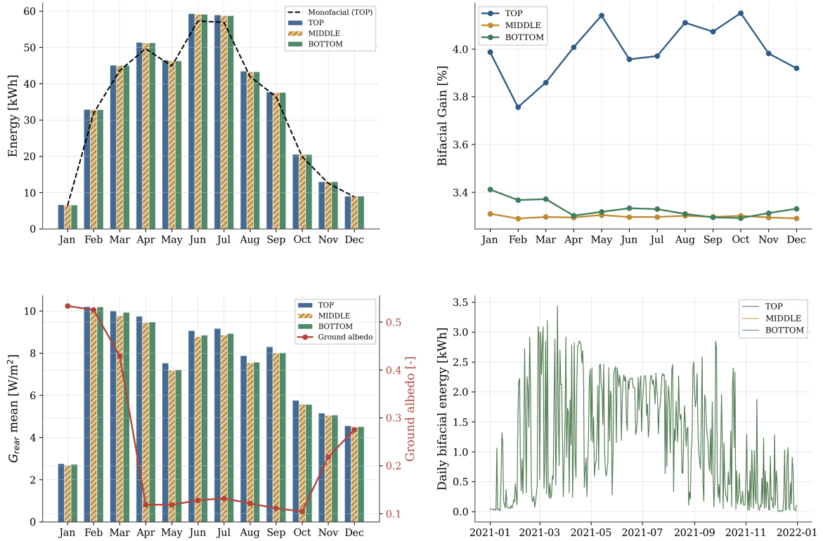
Figure 3: Overview of the annual optical–electrical results for Helsinki Kumpula 2021: (top left) monthly energy yield in the monofacial and bifacial cases for the three positions; (top right) monthly bifacial gain by position; (bottom left) mean rear-side irradiance and monthly ground albedo; (bottom right) daily bifacial energy over the year.
