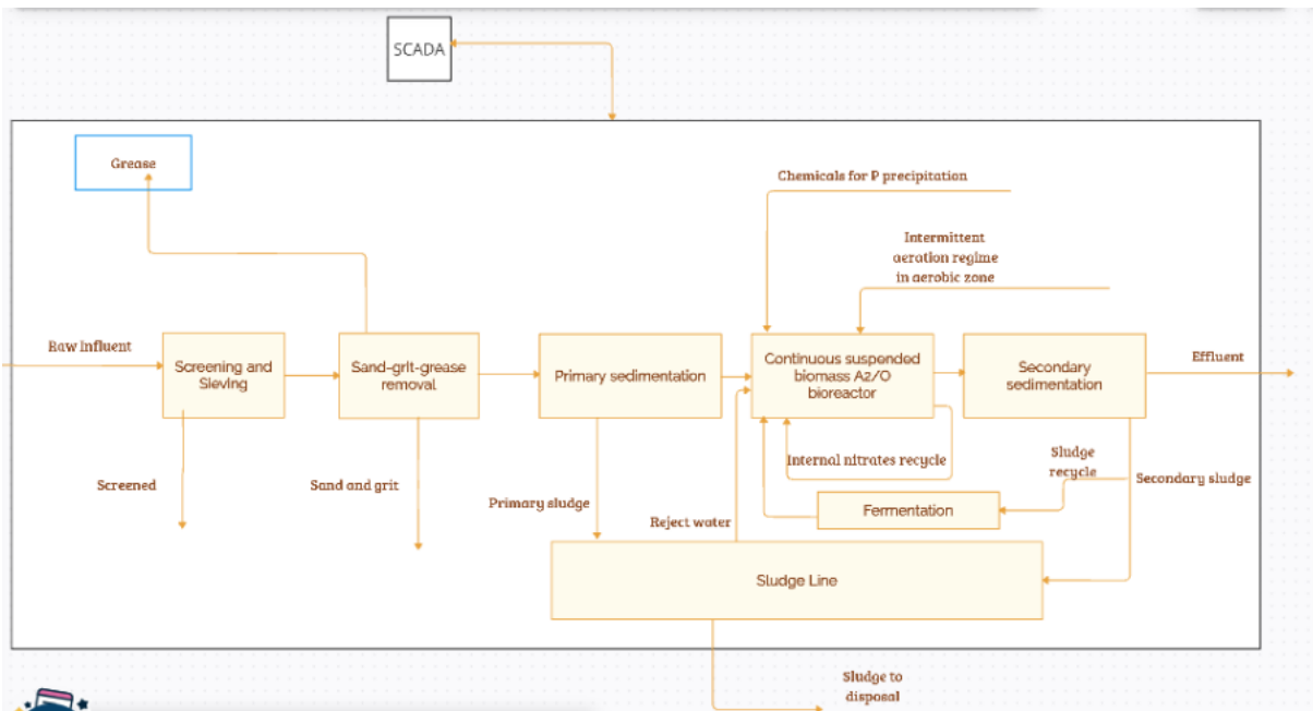
Figure 0.2: Block diagram representative of the water line of group 2 of reference Danish WWTPs
