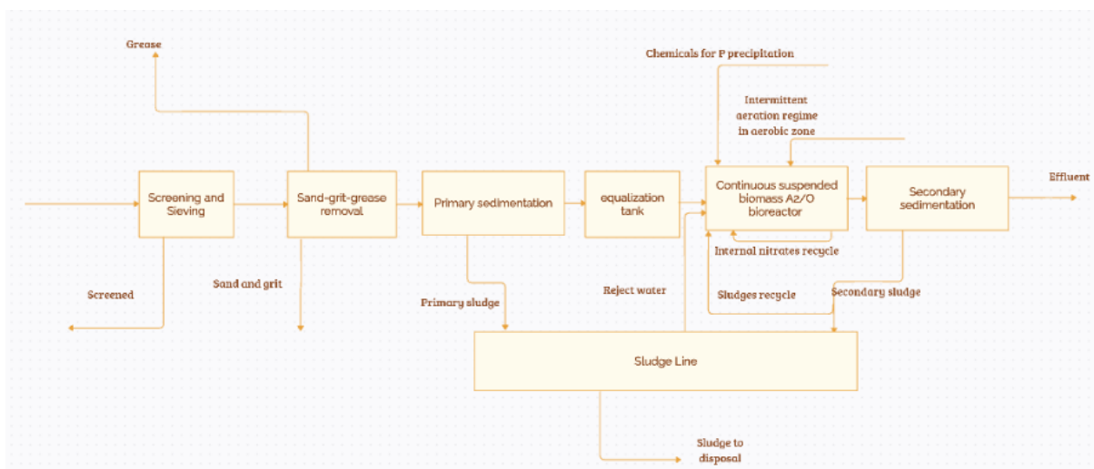
Figure 0.16: Block diagram representative of the water line of group 16 of reference Danish WWTPs
