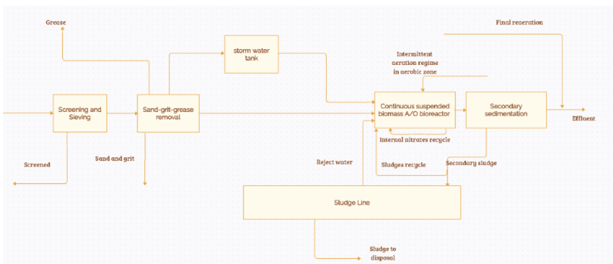
Figure 0.22: Block diagram representative of the water line of group 22 of reference Danish WWTPs
