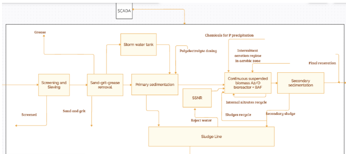
Figure 0.19: Block diagram representative of the water line of group 19 of reference Danish WWTPs
