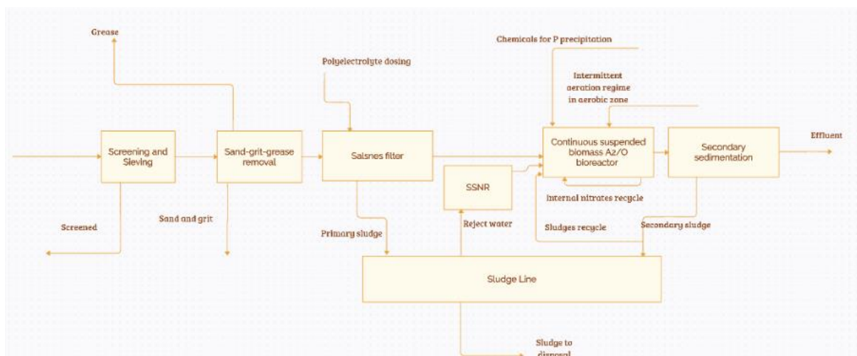
Figure 0.28: Block diagram representative of the water line of group 28 of reference Danish WWTPs
