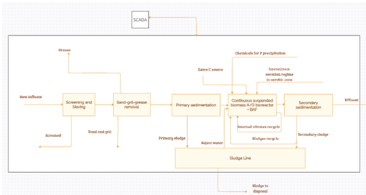
Figure 0.10: Block diagram representative of the water line of group 10 of reference Danish WWTPs
