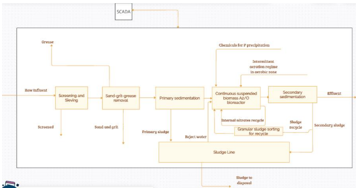
Figure 0.4: Block diagram representative of the water line of group 4 of reference Danish WWTPs
