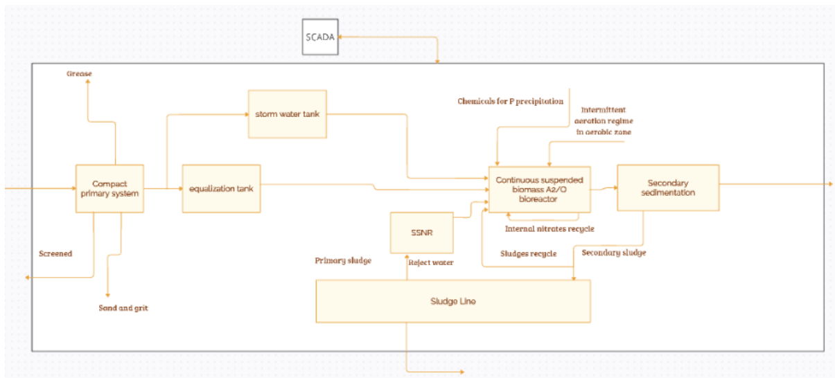
Figure 0.30: Block diagram representative of the water line of group 30 of reference Danish WWTPs
