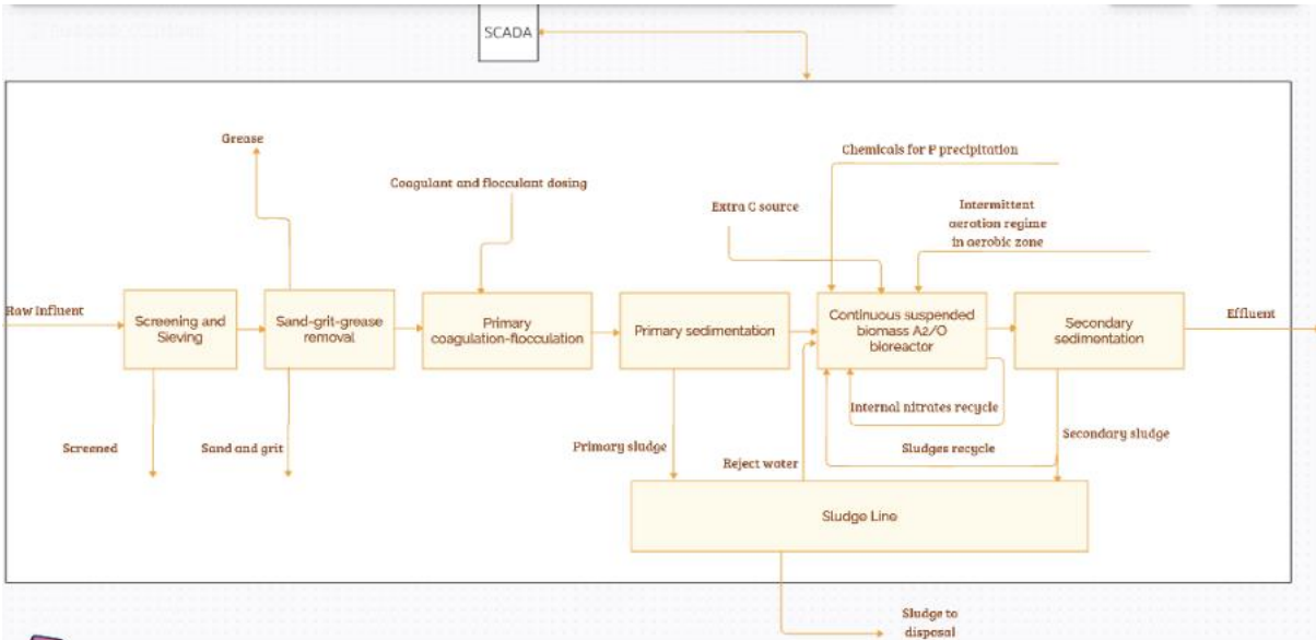
Figure 0.1: Block diagram representative of the water line of group 1 of reference Danish WWTPs
