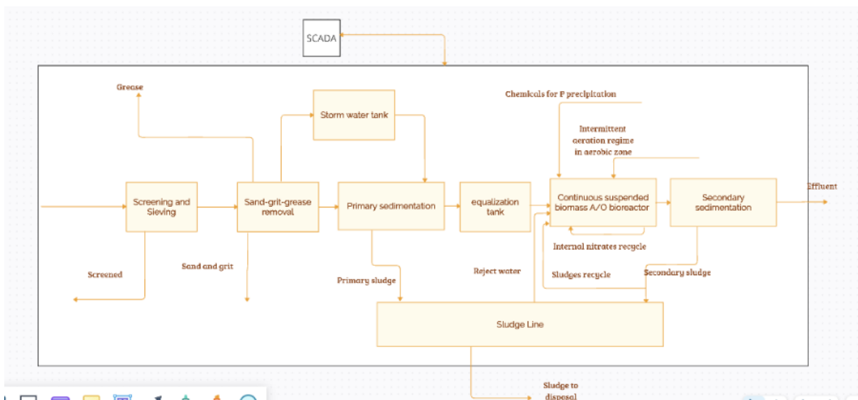
Figure 0.12: Block diagram representative of the water line of group 12 of reference Danish WWTPs
