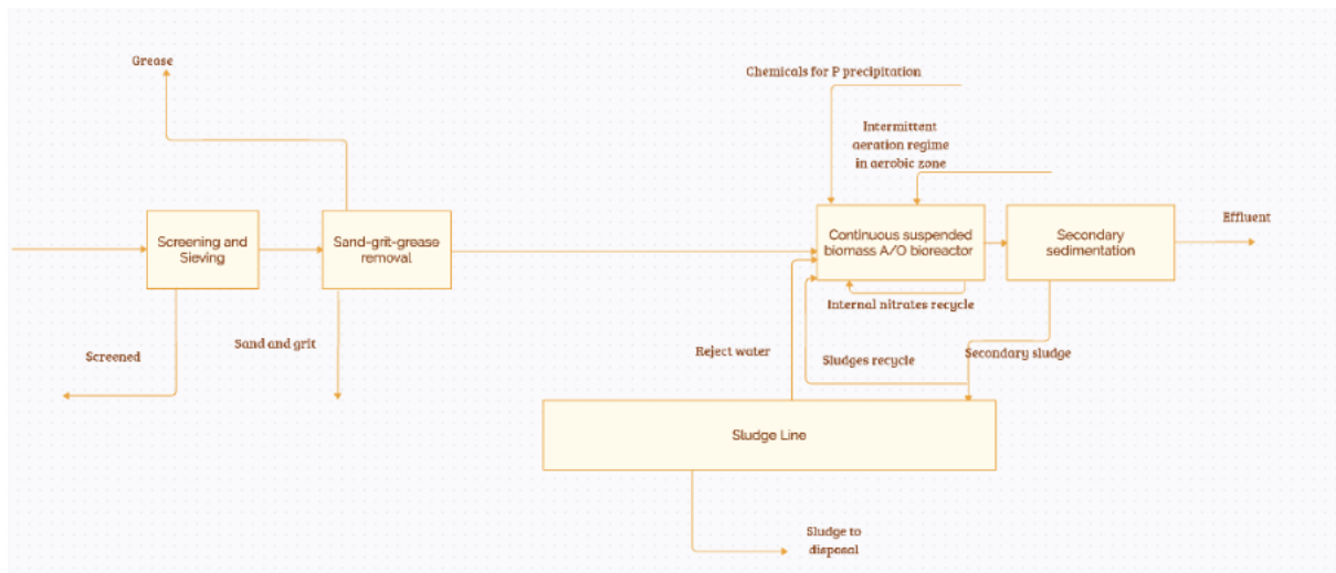
Figure 0.26: Block diagram representative of the water line of group 26 of reference Danish WWTPs
