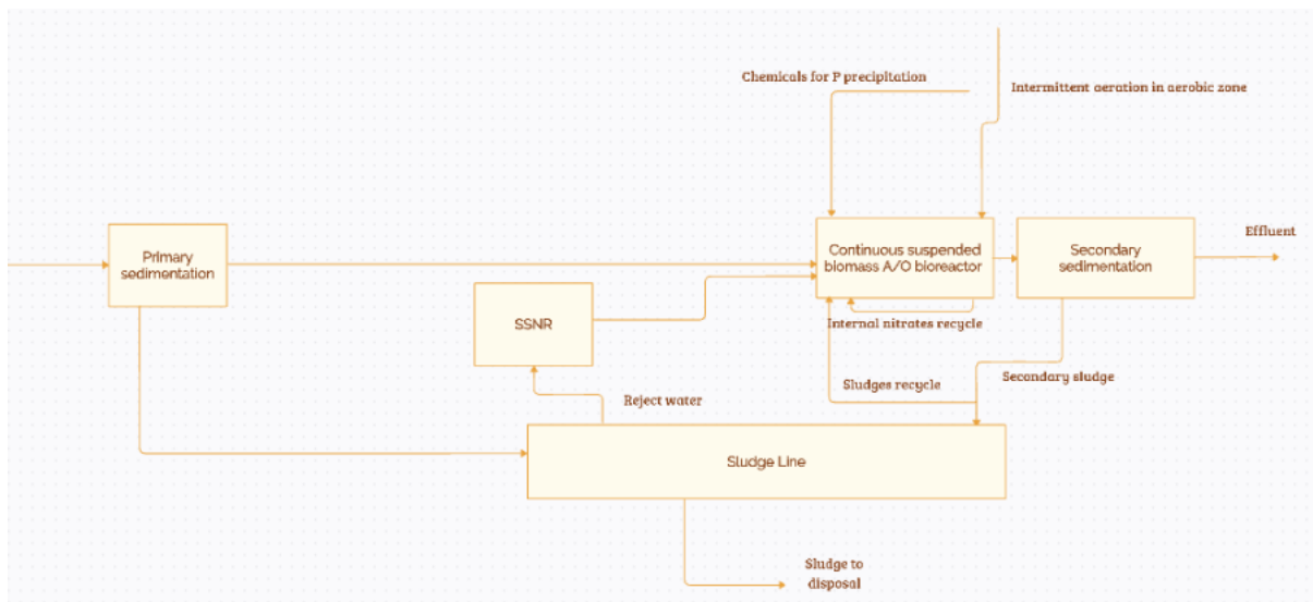
Figure 0.31: Block diagram representative of the water line of group 31 of reference Danish WWTPs
