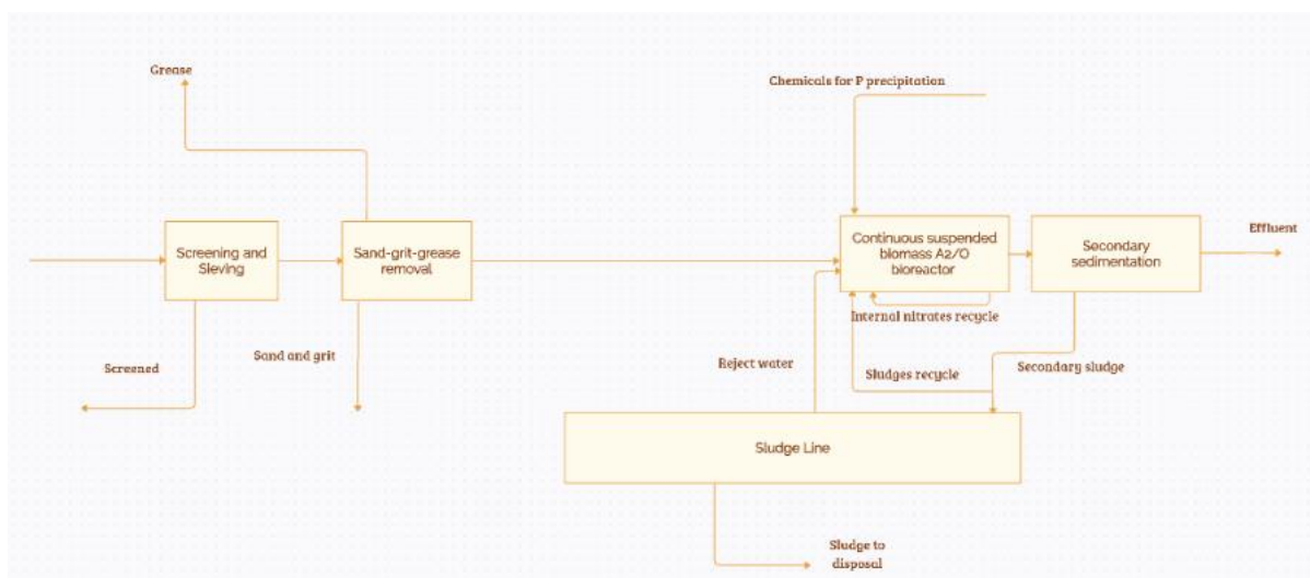
Figure 0.24: Block diagram representative of the water line of group 24 of reference Danish WWTPs
