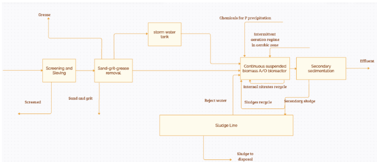
Figure 0.21: Block diagram representative of the water line of group 21 of reference Danish WWTPs
