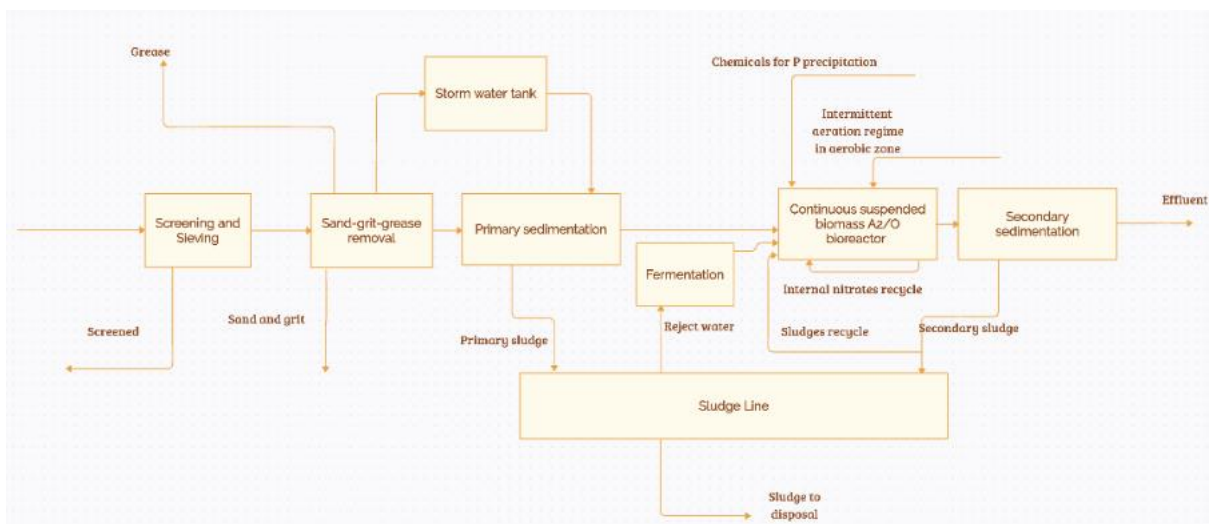
Figure 0.18: Block diagram representative of the water line of group 18 of reference Danish WWTPs
