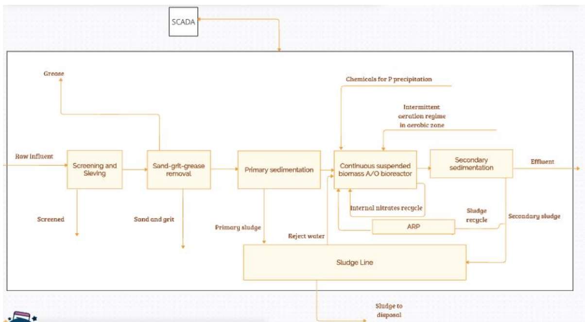
Figure 0.8: Block diagram representative of the water line of group 8 of reference Danish WWTPs
