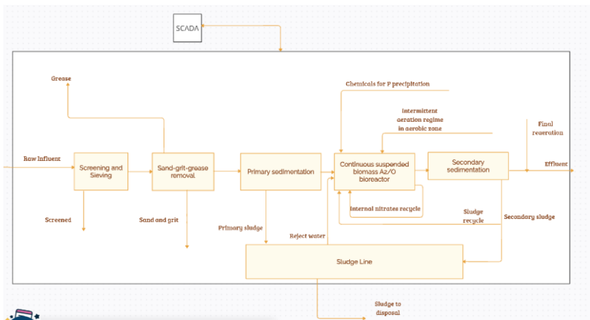
Figure 0.3: Block diagram representative of the water line of group 3 of reference Danish WWTPs
