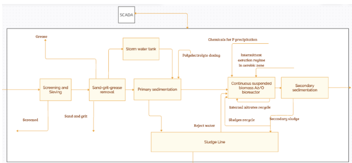
Figure 0.20: Block diagram representative of the water line of group 20 of reference Danish WWTPs
