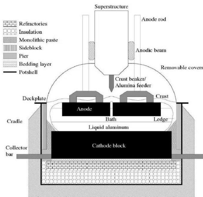
Figure 2.7 : Diagram of a standard Hall-Héroult electrolysis cell [139]
