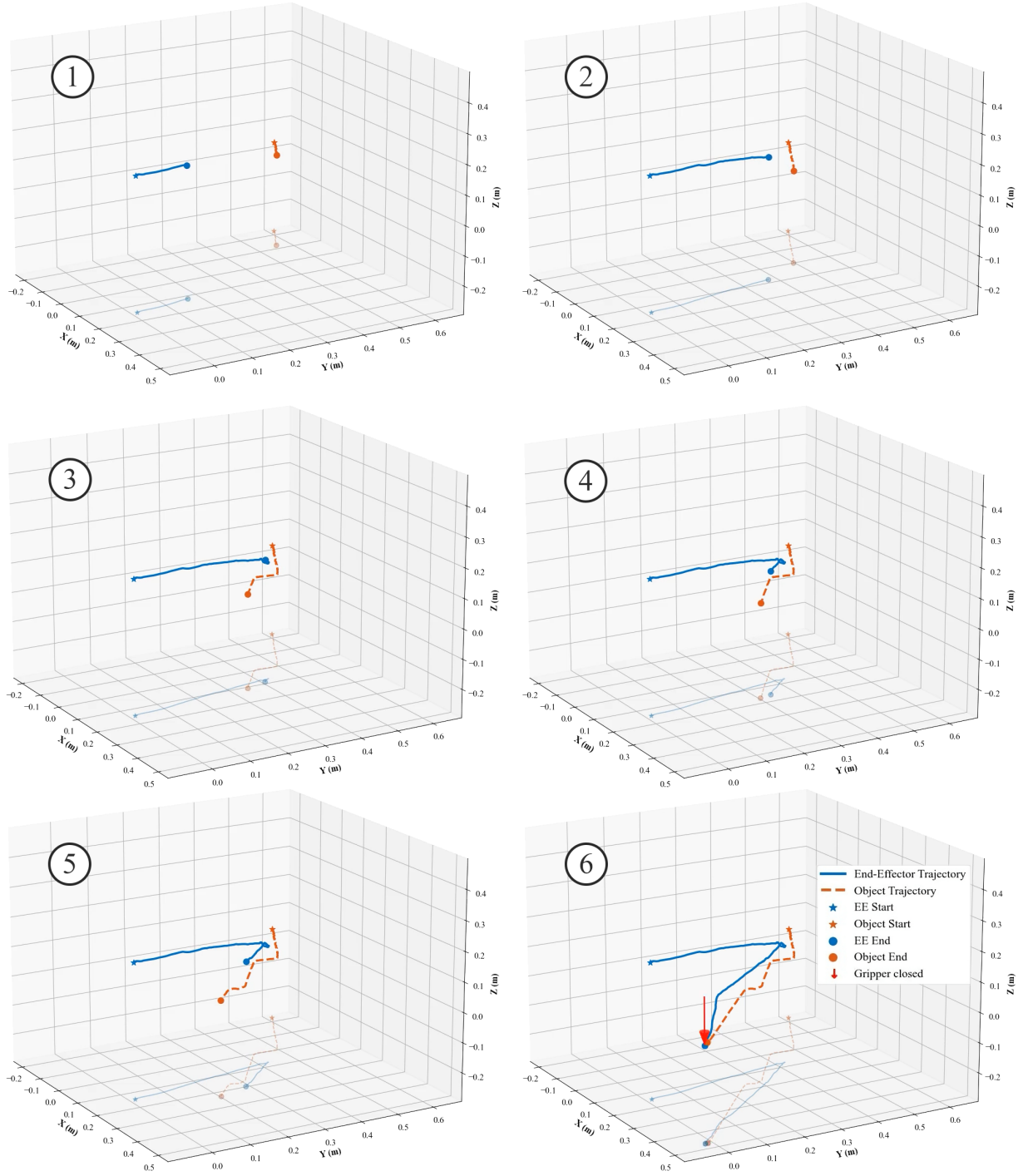
Figure 37: End-effector (solid) and object (dashed) 3D trajectories in the direction-change test performed at a relative speed of 0.10 \text{ m/s} .
