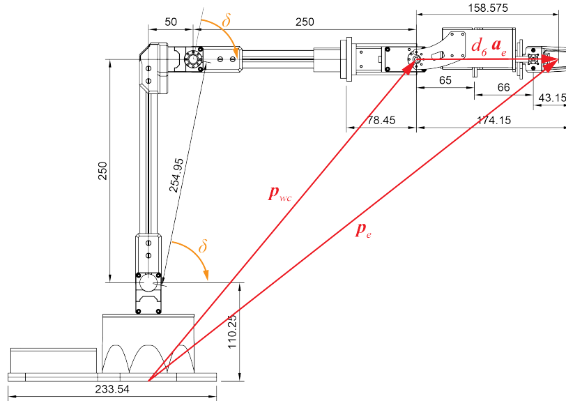
Figure 3: Wrist-center position vector \mathbf{p}_{wc} from the end-effector pose \mathbf{p} .
